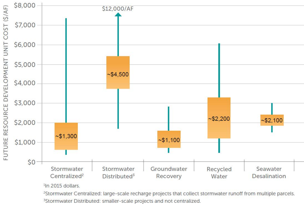
Figure 2-1. Summary of Future Resource Development Unit Costs 1
