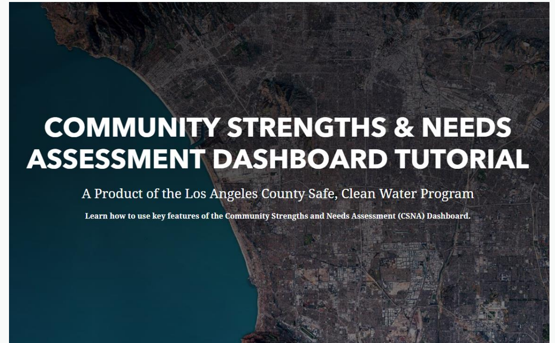
Dashboard Tutorial
