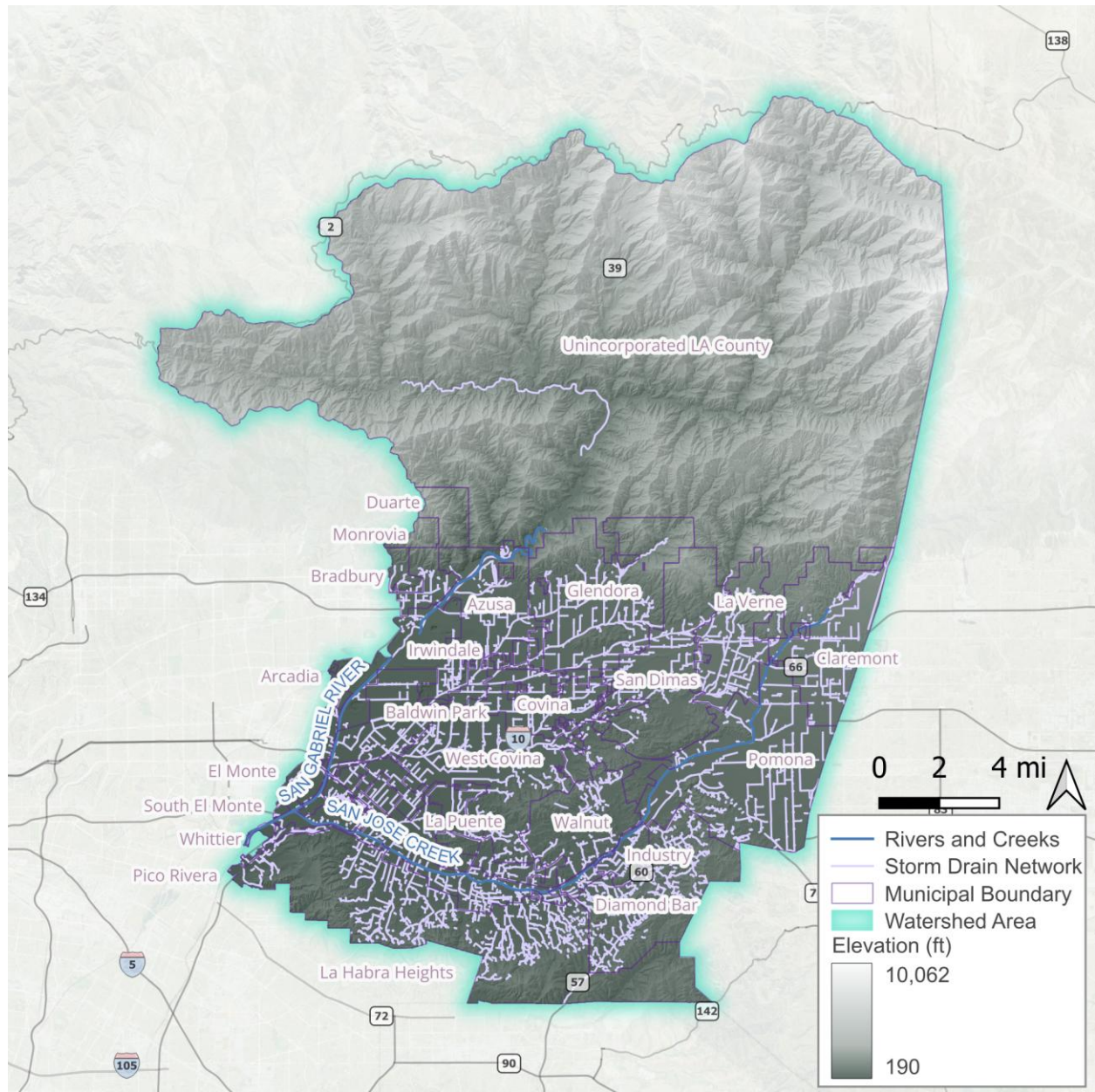
Figure 2-3. USGR WA elevation profile
