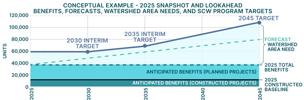
Figure 3-5. Conceptual example illustrating benefits, WA Needs, targets, and forecasts
