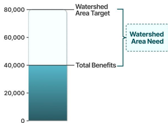
Figure 5-2. WA Need conceptual example for a magnitude-based Indicator
