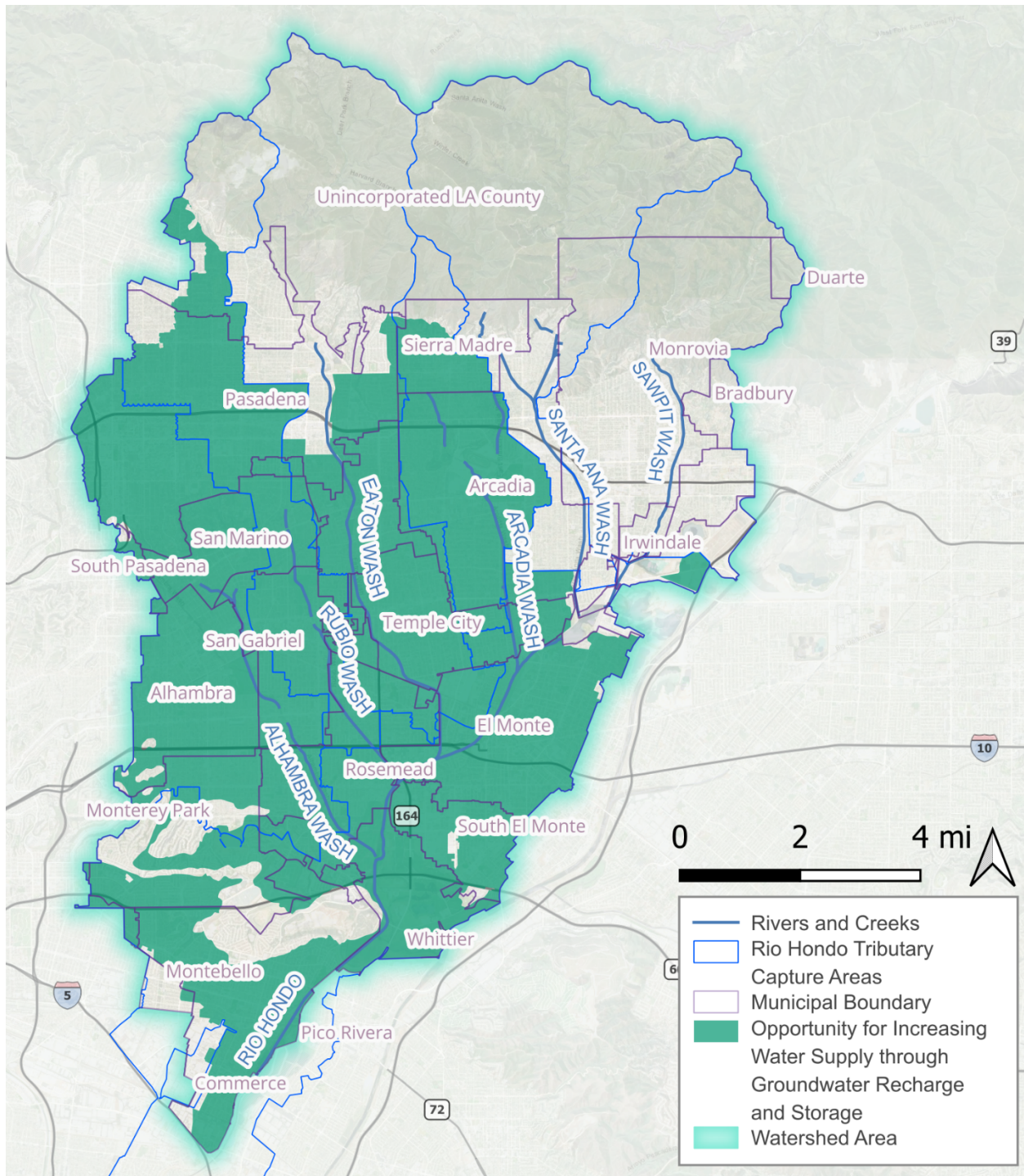
Figure I-6. Opportunity to Increase Water Supply Through Groundwater Recharge and Storage
